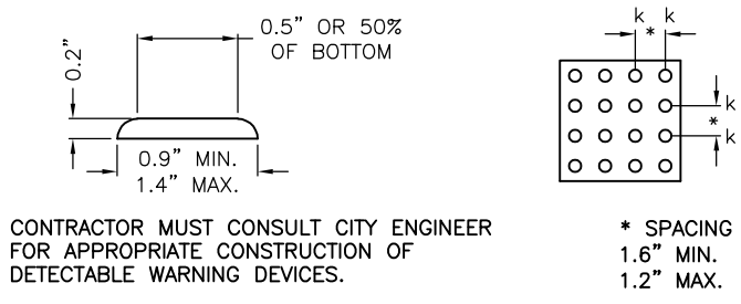
DETECTABLE WARNING DETAIL - RAISED TRUNCATED DOMES -
