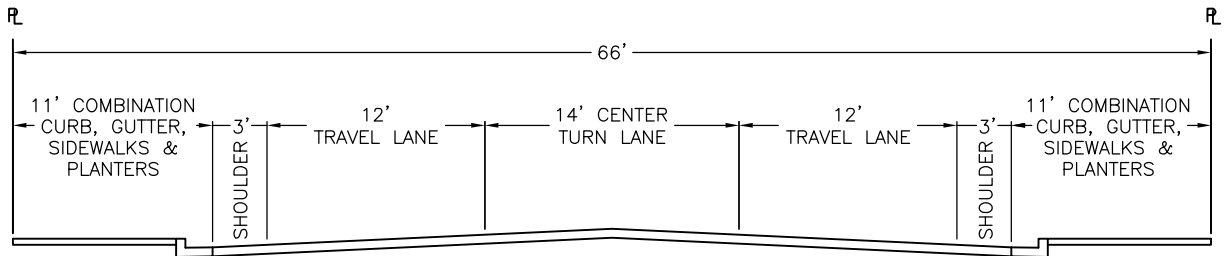
MINOR COLLECTOR - 66' RIGHT-OF-WAY
