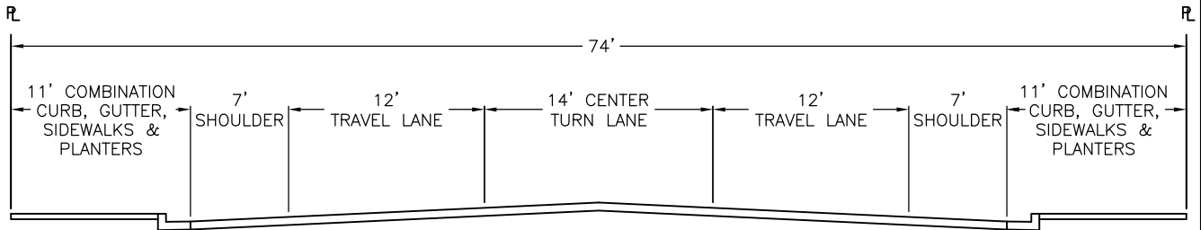
MAJOR COLLECTOR - 74' RIGHT-OF-WAY
