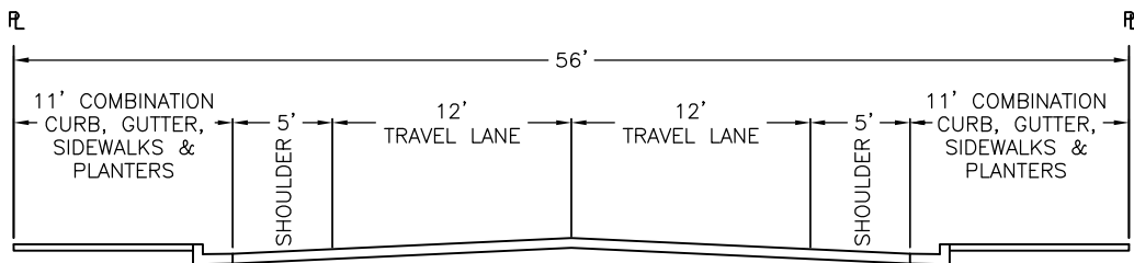
LOCAL - 56' RIGHT-OF-WAY
